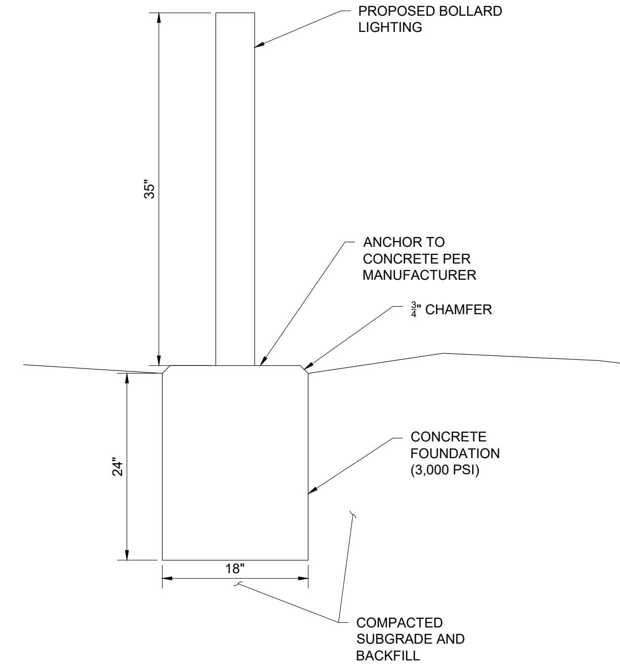
BOLLARD INSTALLATION DETAIL INSTALL PER MANUFACTURER'S INSTRUCTIONS AND REQUIREMENTS
